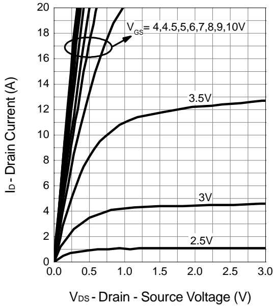
Output Characteristics
