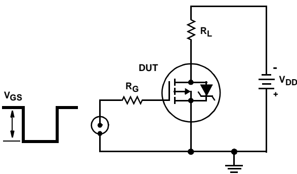
FIGURE 39. SWITCHING TIME TEST CIRCUIT
