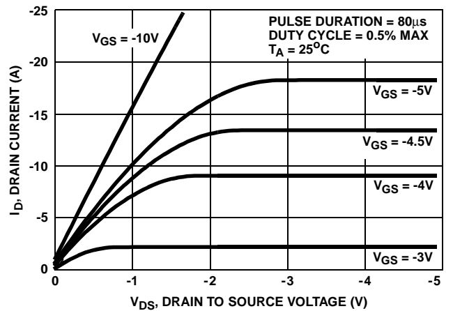
FIGURE 28. SATURATION CHARACTERISTICS
