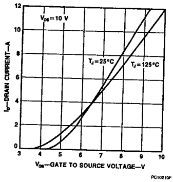
Figure 5 Transfer Characteristics
