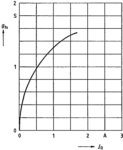
Typical transconductance g_{fs} = f(I_D)
