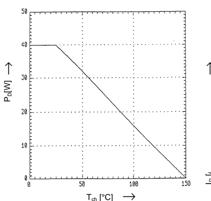
Power Dissipation
