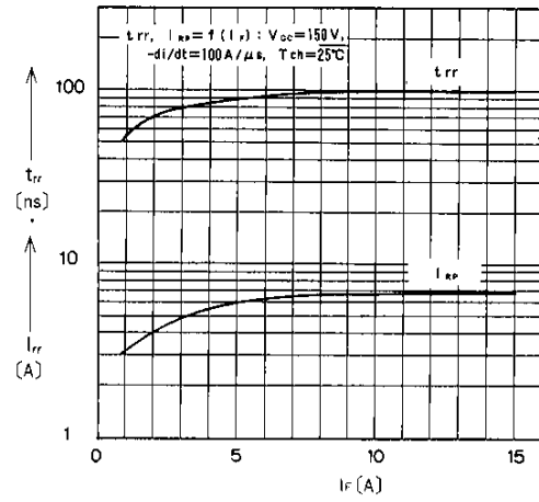
Reverse Recovery Characteristics
