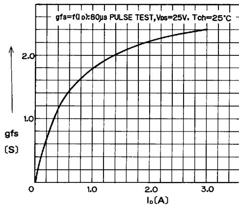
Typical Forward Transconductance vs. I_D
