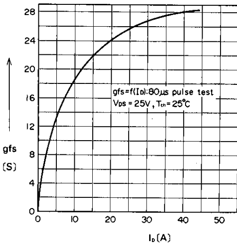
Typical Forward Transconductance vs. I_D
