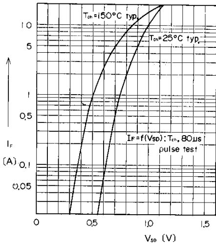
Forward Characteristics of Reverse Diode
