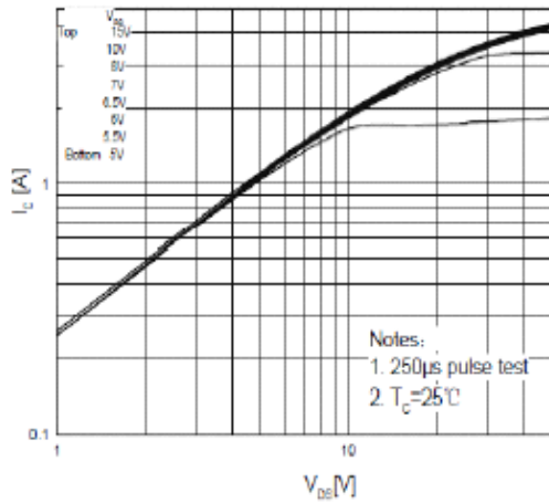
Fig.1 On-State Characteristics
