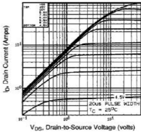
Fig.1 On-state Characteristics
