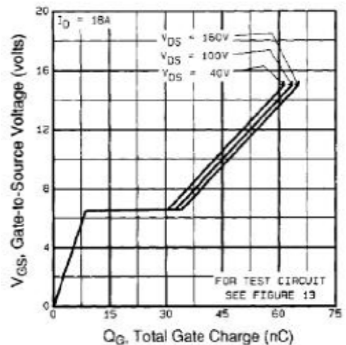
Fig.6 Gate Charge Characteristics
