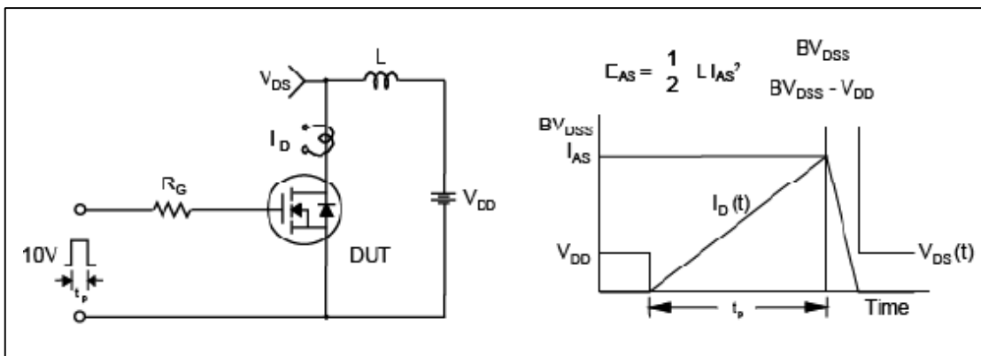
Fig.12 Uncamped Inductive Switching Test Circuit & Waveform
