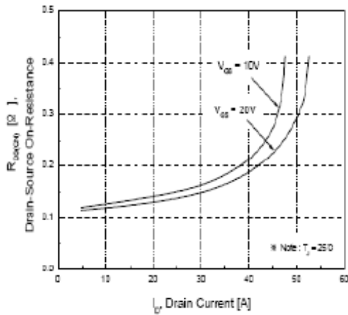
Fig.3 On-Resistance Variation vs Drain Current
