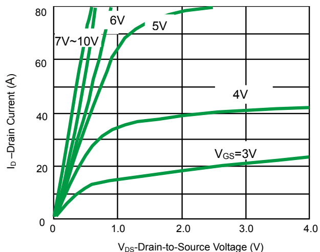
Fig 6. On-Region Characteristics
