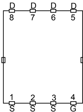
Top View (PDFN5*6-8L)
