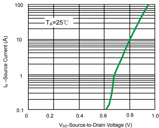
Fig 8. Source to Drain Diode Forward Voltage
