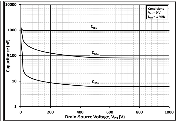
Figure 14. Typical Typical Capacitances vs. Drain-Source Voltage (0 - 1000V)
