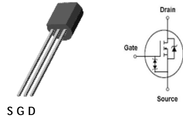
TO-92
