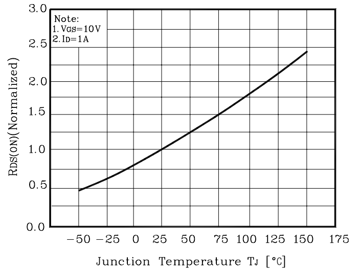
Fig. 8 R_{DS(on)} - T_J
