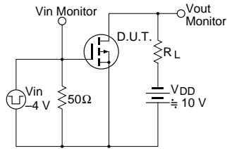
Switching Time Test Circuit
