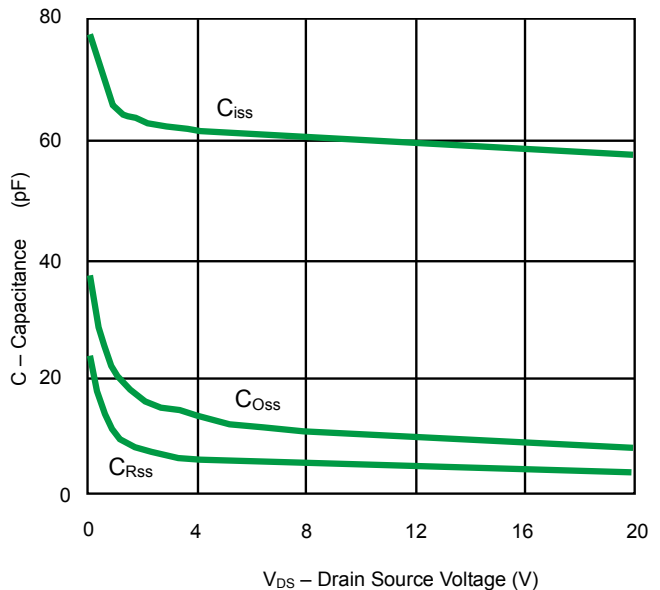
Fig 4. Capacitance
