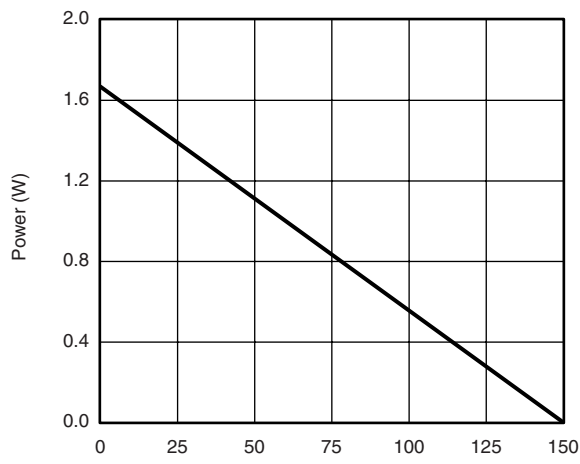
T_C - Case Temperature ( ^\circ\text{C} ) Power Derating, Junction-to-Foot
