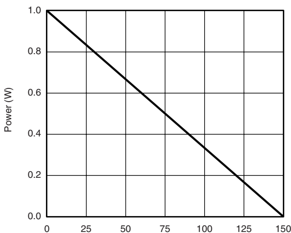
T_A - Ambient Temperature ( ^\circ\text{C} ) Power Derating, Junction-to-Ambient
