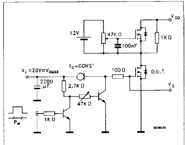
Fig. 2: Gate Charge Test Circuit
