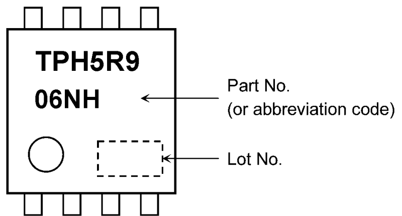
Fig. 7.1 Marking
