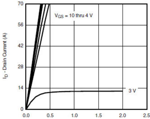
Output Characteristics
