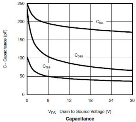
Capacitance
