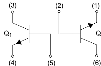
BC847CDXV6T1
