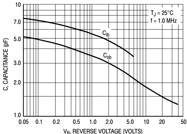
Figure 15. Capacitance
