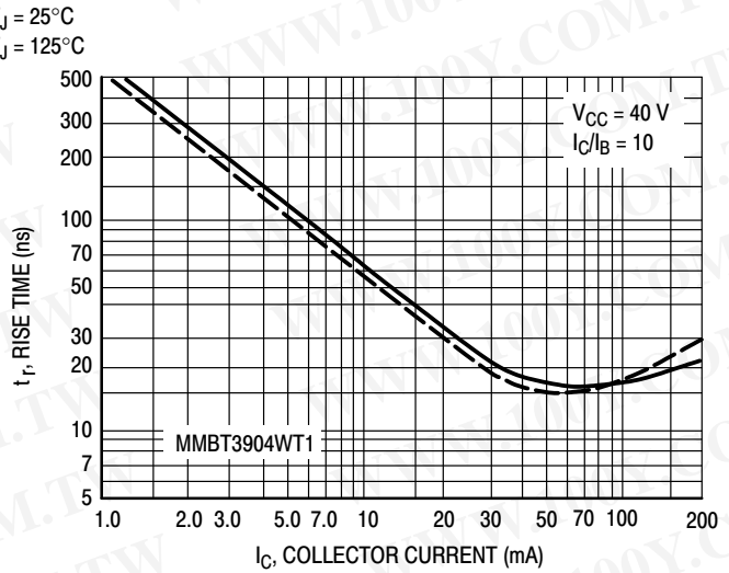
Figure 4. Rise Time
