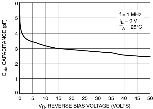
Figure 44. Output Capacitance
