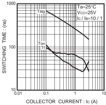
Fig.1 Switching Time
