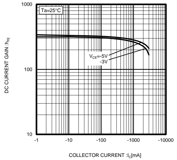
Fig.2 DC Current Gain vs. Collector Current ( I )
