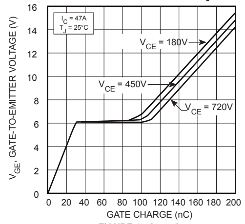
FIGURE 4, Gate charge
