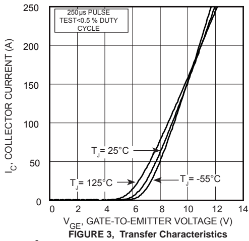
FIGURE 3, Transfer Characteristics
