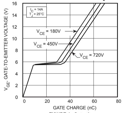
FIGURE 4, Gate charge
