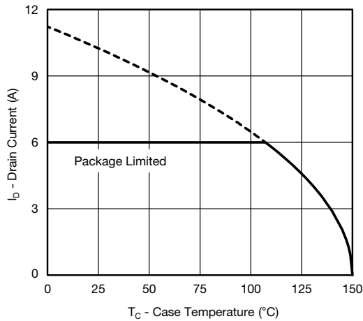
Current Derating*
