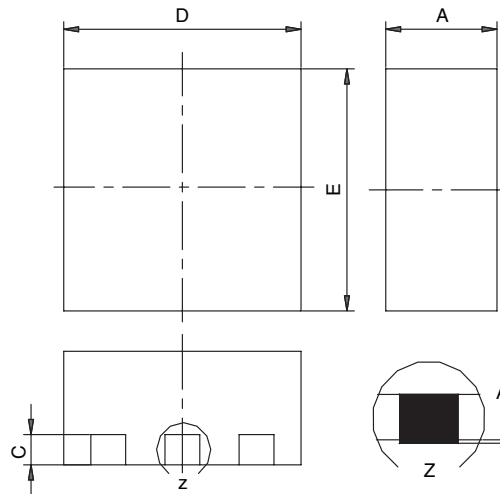
DETAIL Z
