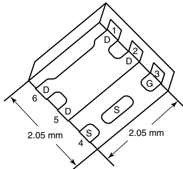
PowerPAK SC-70-6L-Single
