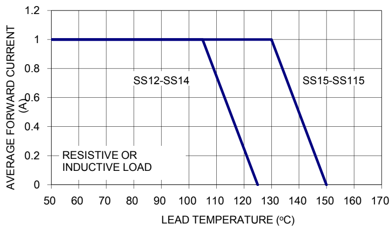
FIG.1 FORWARD CURRENT DERATING CUURVE
