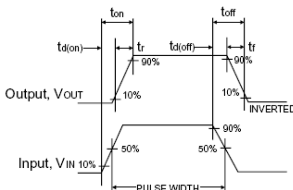
Switchin Waveforms
