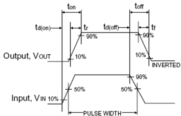
Switchin Waveforms
