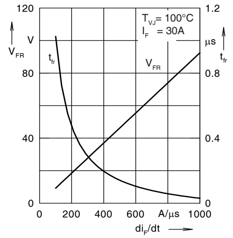
Fig. 18. Peak forward voltage V_{FR} and t_{tr} versus di_F/dt
