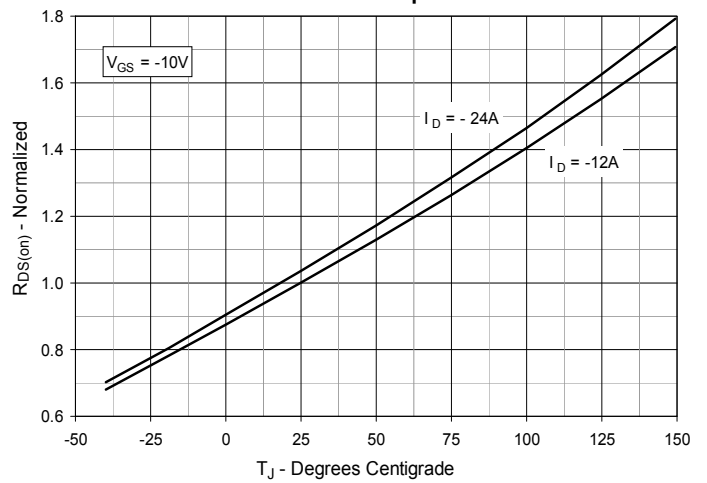
Fig. 4. R_{DS(on)} Normalized to I_D = -12\text{A} vs. Junction Temperature
