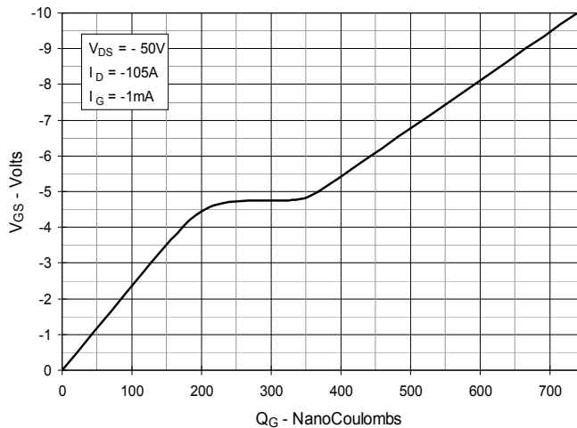
Fig. 10. Gate Charge
