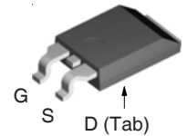
PLUS220SMD (IXTV_S)
