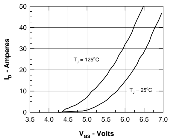
Figure 6. Admittance Curves
