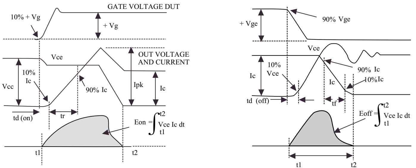
Fig 22. Definition Switching Time & Loss
