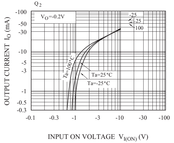
I_O - V_{I(ON)}
