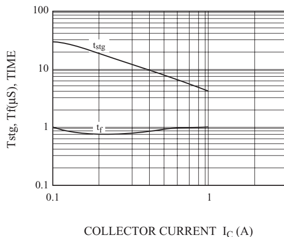
SWITCHING TIME
