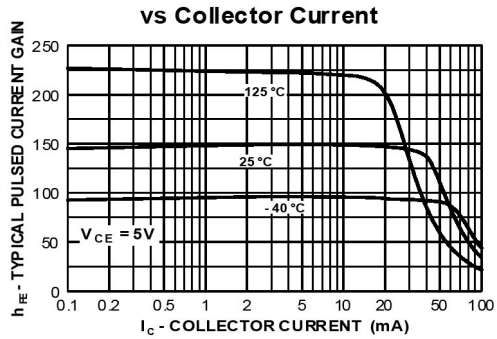
Figure 1. Typical Pulsed Current Gain vs Collector Current
