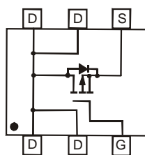
Top View Internal Schematic
