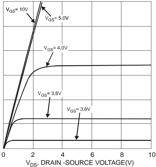
Figure 1 Typical Output Characteristics
