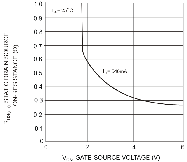
Fig. 6 Static Drain-Source, On-Resistance vs. Gate-Source Voltage
