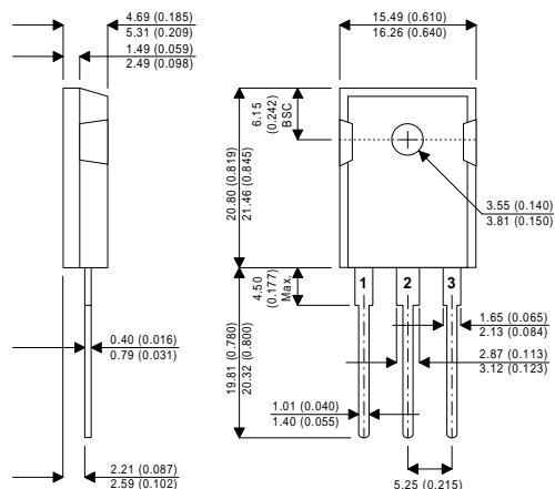
TO-247
